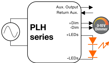
Application Diagram
