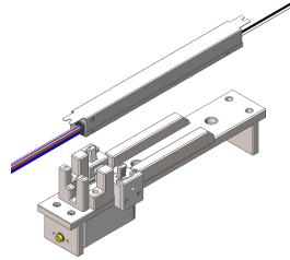
Programming Cradle Part number: PROG-PLH-CRADLE
