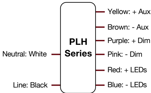
Wiring Diagram
